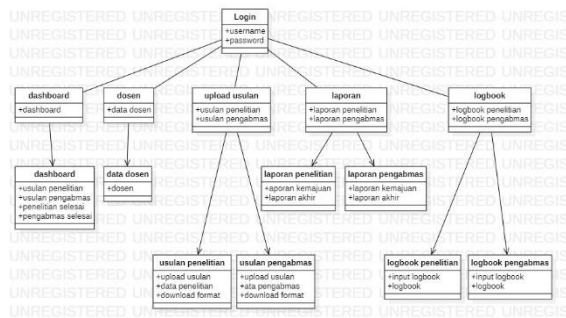
Gambar 34 Class Diagram
