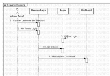
Gambar 35 Sequence Diagram Login
